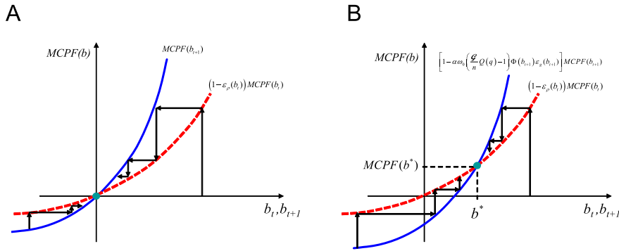
Fig. 1. The Euler equation for G = q = n and q < n .
