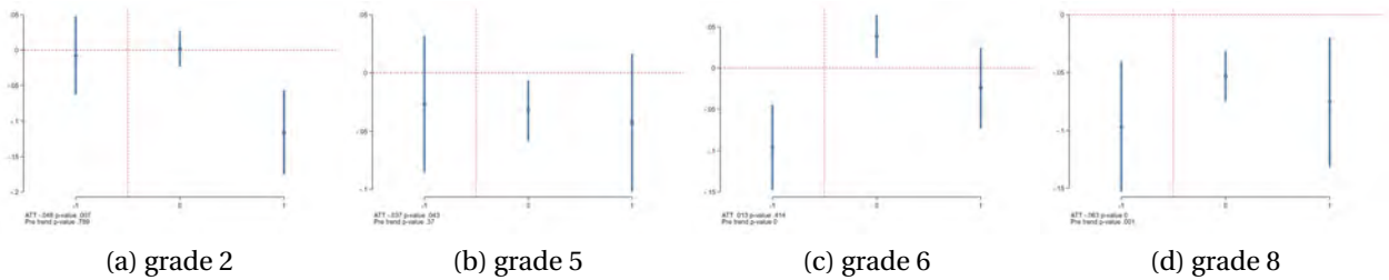
Figure A6. Standardize score literacy
